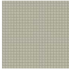
Vanadio OPS 2006
