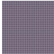
Pirrotina OPS 2011
