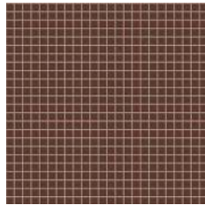
Ferro OPS 2010
